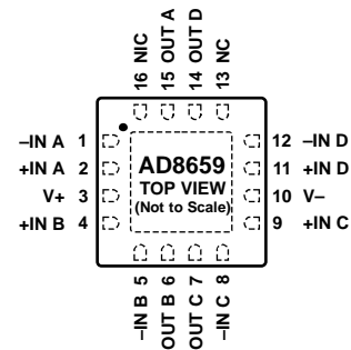
NOTES 1. NIC = NO INTERNAL CONNECTION. 2. CONNECT THE EXPOSED PAD TO V- OR LEAVE IT UNCONNECTED.
