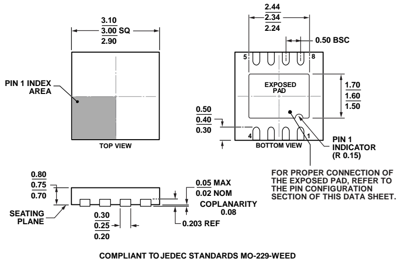
Figure 80. 8-Lead Lead Frame Chip Scale Package [LFCSF_WD] 3 mm x 3 mm Body, Very Very Thin, Dual Lead (CP-8-11) Dimensions shown in millimeters
