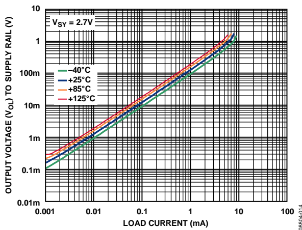
Figure 22. Output Voltage ( V_{OL} ) to Supply Rail vs. Load Current
